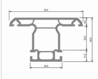
JPI UPVC Sliding & Casement Mullion YTB 77 109
