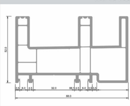
SLIDER FRAME WITH MESH TRACK YTB 78 105
