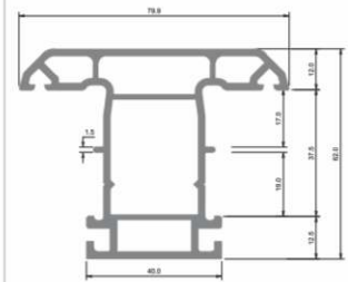
Prominance UPVC Casement Mullion YTB 77 105
