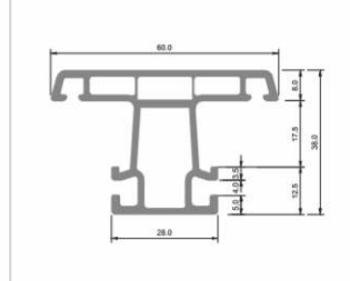
Simta UPVC Sliding & Casement Mullion YTB 77 106
