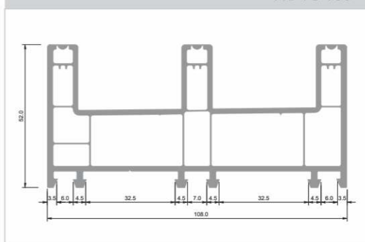
SLIDER FRAME 3- TRACK YTB 78 106
