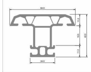
Prominance UPVC Sliding & Casement Mullion YTB 77 110
